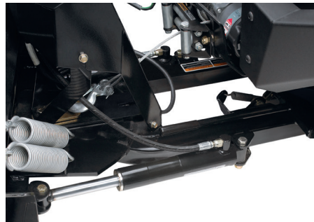
Dual cylinders hydraulic
